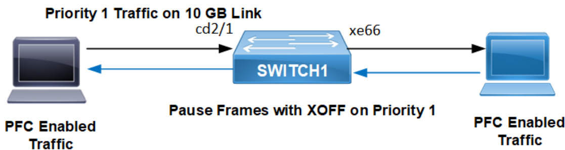
Figure 6. PFC Enabled Bridge
