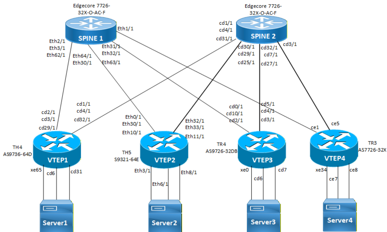
Figure 4. PFC Dead Lock Detection and Recovery
