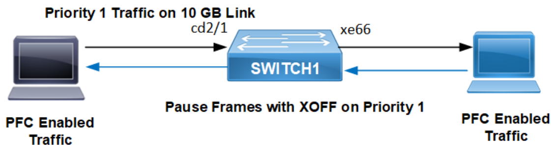
Figure 165. PFC Enabled Bridge
