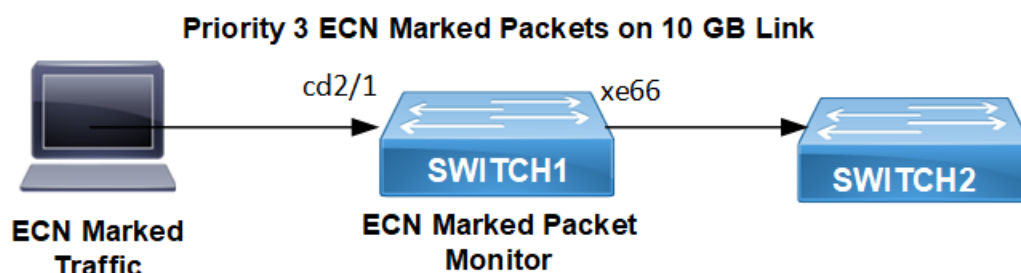
Figure 166. ECN Enabled Bridge
