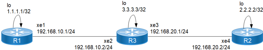
Figure 84. Configure Overload Bit Suppress
