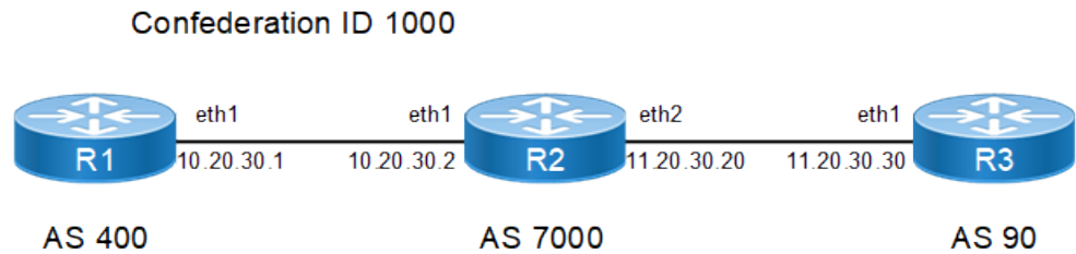
Figure 19. BGP Confederation
