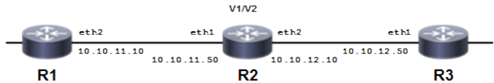
Figure 137. RIP Version Topology
