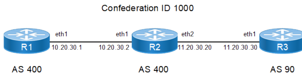
Figure 20. BGP Confederation with Multiple AS
