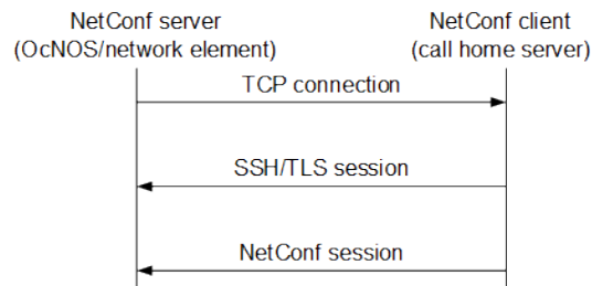
Figure 57. RFC 8071 NetConf call home functionality
