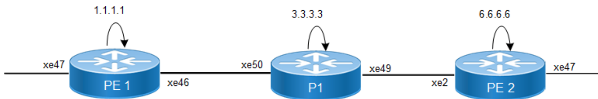
Figure 65. ACL on IRB sample topology
