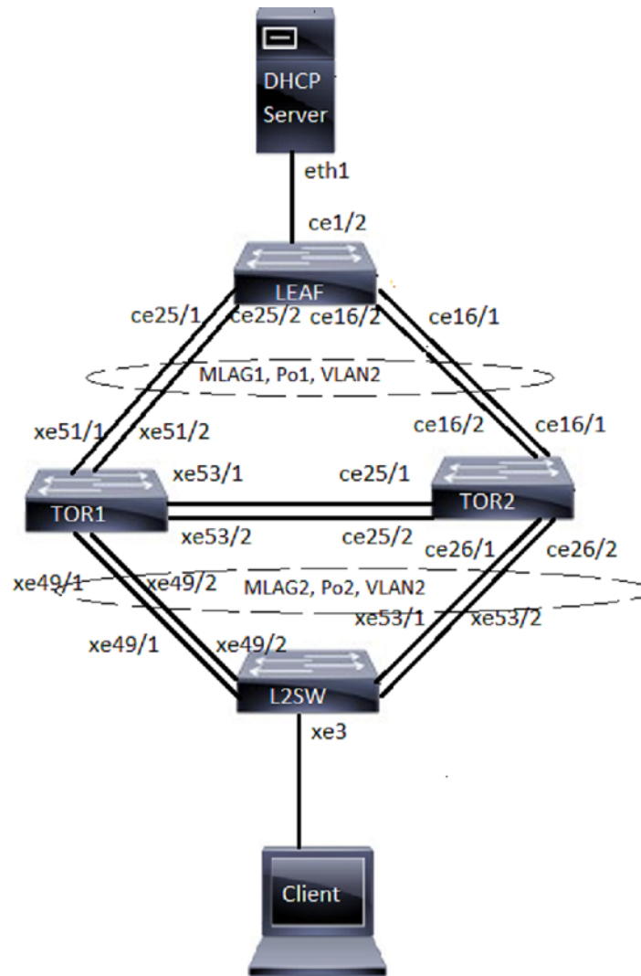
Figure 71. DHCP Snooping over MLAG
