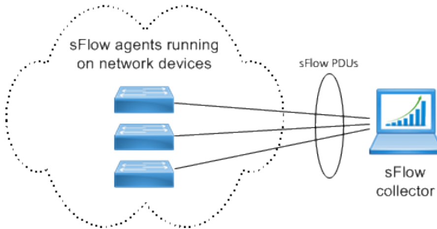
Figure 47. Basic sFlow topology
