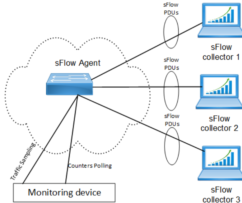
Figure 48. sFlow with Multiple Collectors
