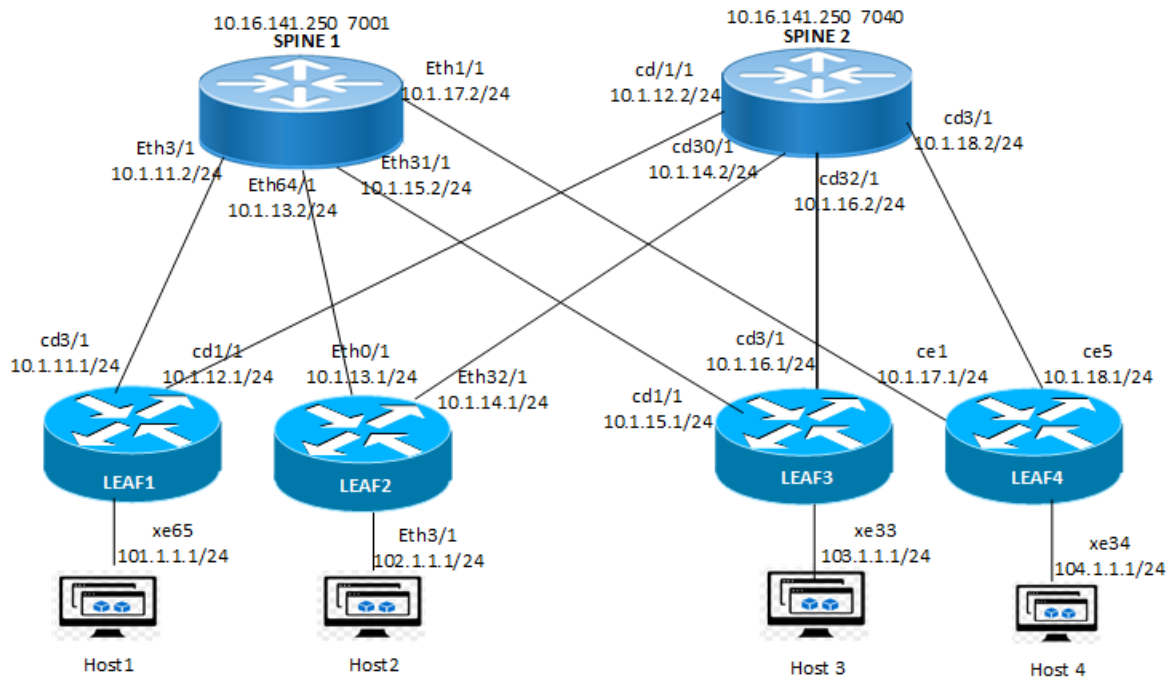
Figure 76. DLB Topology
