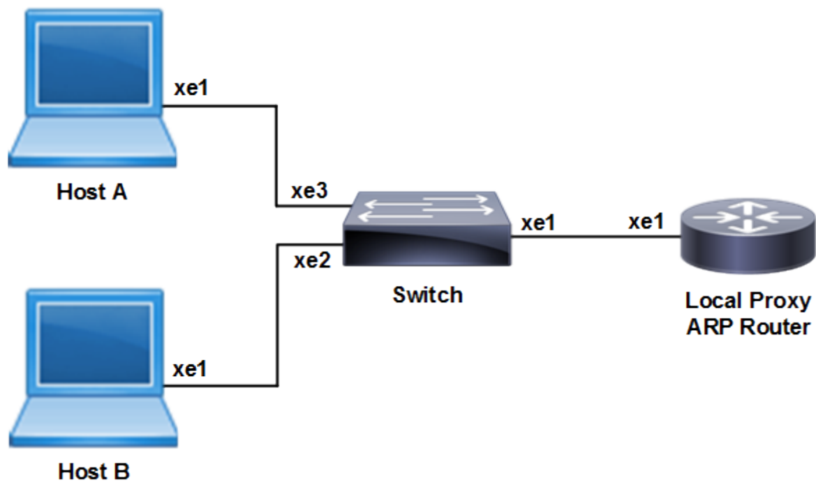
Figure 68. Sample topology
