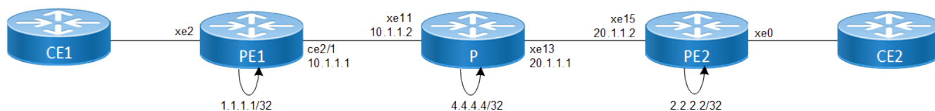
Figure 65. MPLS Layer 2 Virtual Circuit
