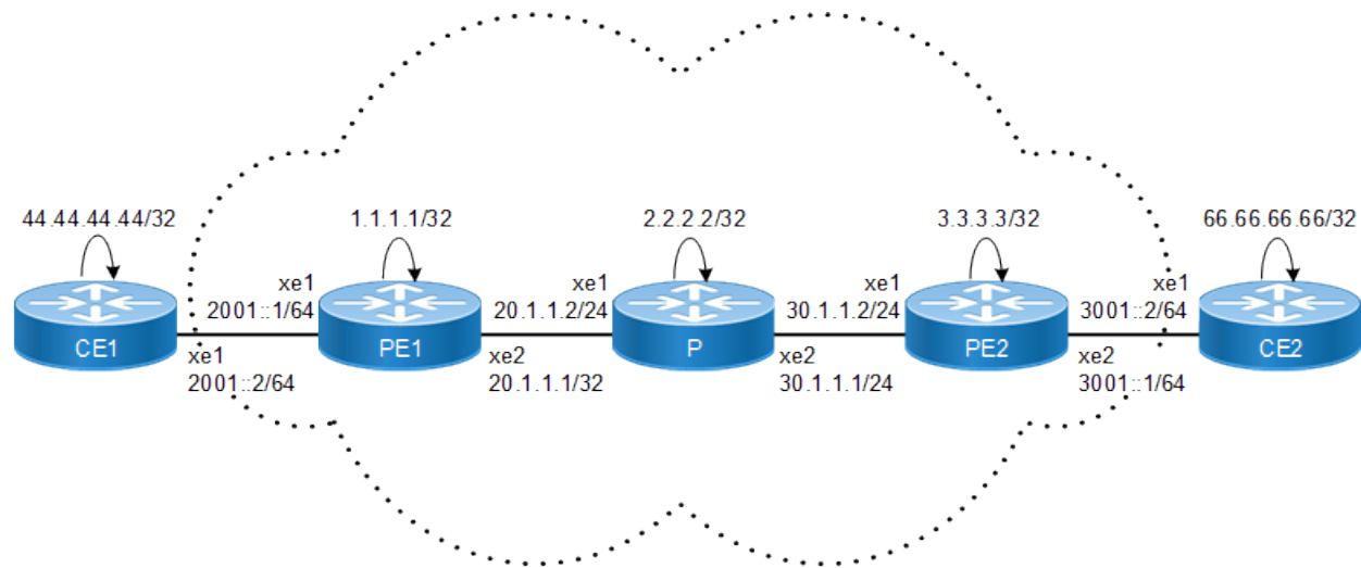
Figure 104. 6PE Configuration
