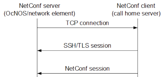
Figure 69. RFC 8071 NetConf call home functionality
