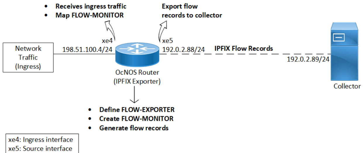
Figure 60. IPFIX Exporter
