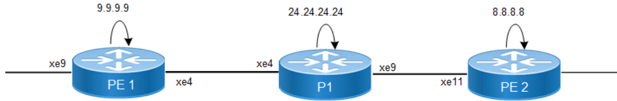
Figure 77. ACL on IRB sample topology
