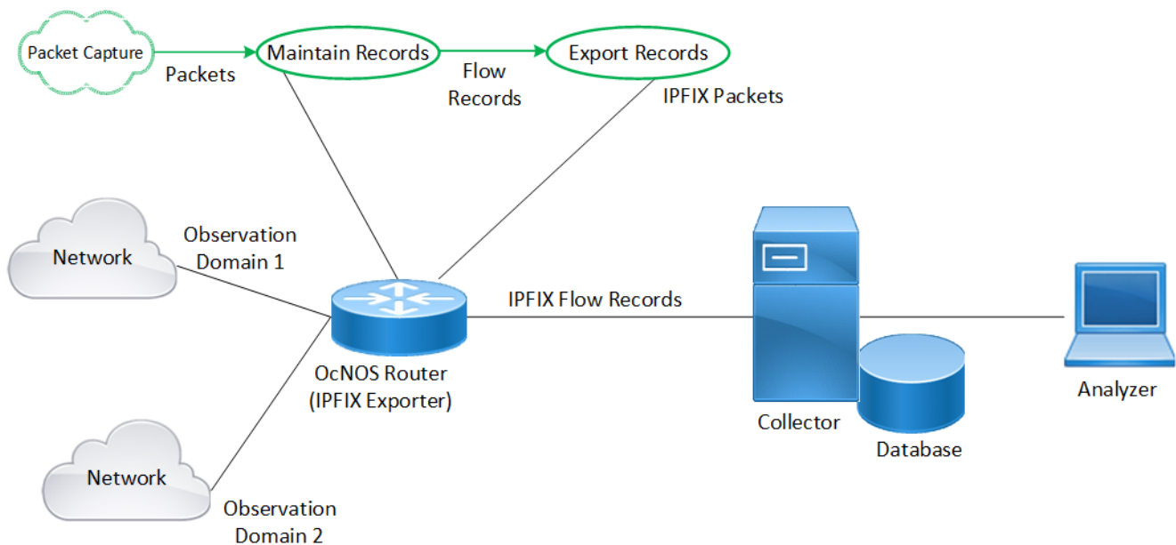
Figure 59. IPFIX Exporter
