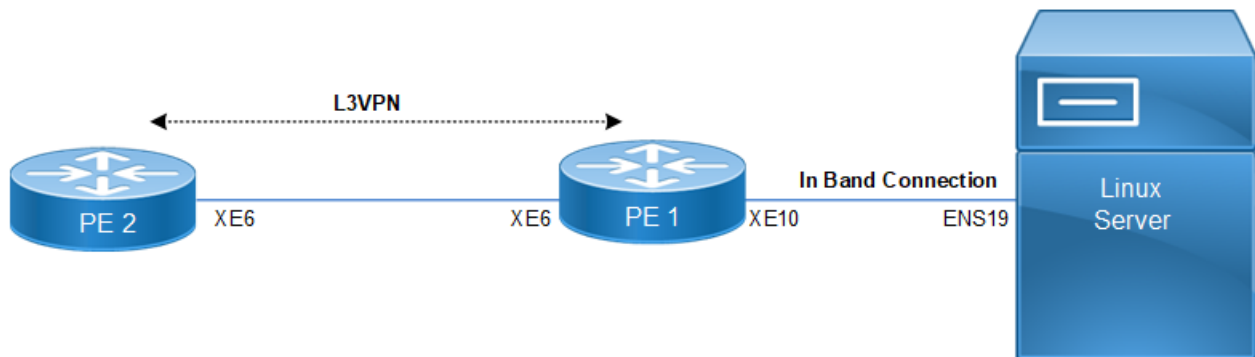
Figure 24. Custom VRF
