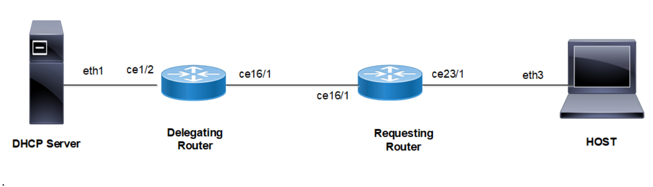
Figure 36. DHCPv6 Relay Delegating Configuration
