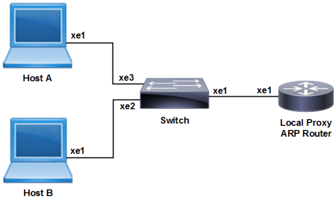
Figure 78. Sample topology
