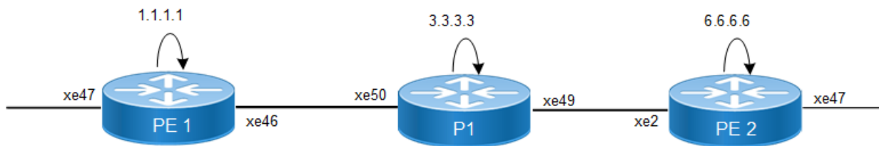
Figure 74. ACL on IRB sample topology
