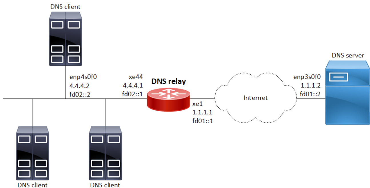
Figure 34. DNS relay configuration
