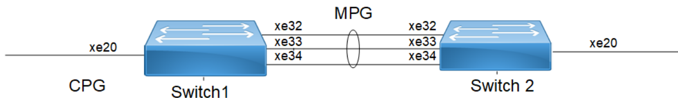
Figure 60. TFO with port-channel
