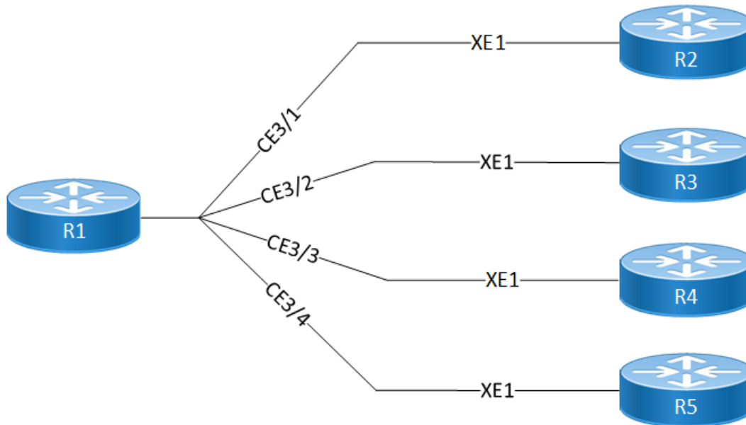
Figure 84. Qumran 2 100G Port Breakout
