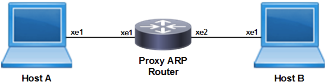
Figure 77. Sample topology
