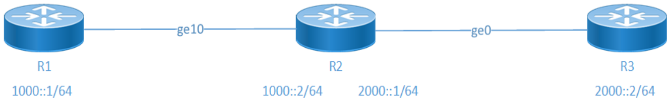
Figure 82. No IPv6 Unreachable
