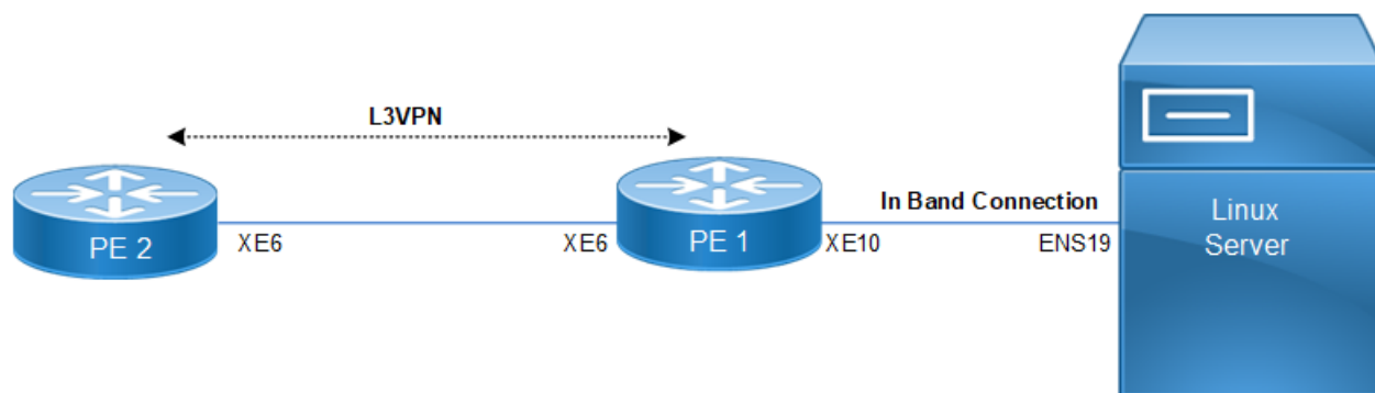
Figure 20. Custom VRF
