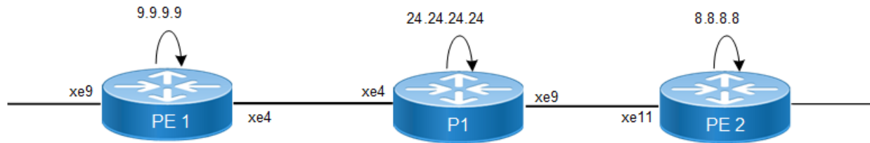
Figure 73. ACL on IRB sample topology
