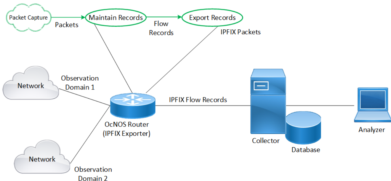
Figure 55. IPFIX Exporter
