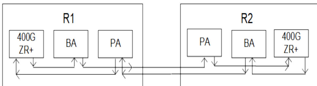
Figure 64. EDFA Sample Topology
