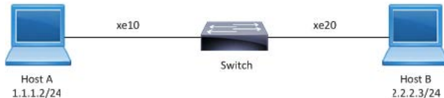
Figure 73. ACL sample topology
